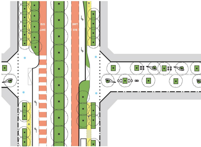
Figure 8 Raised pedestrian and cycle crossing
