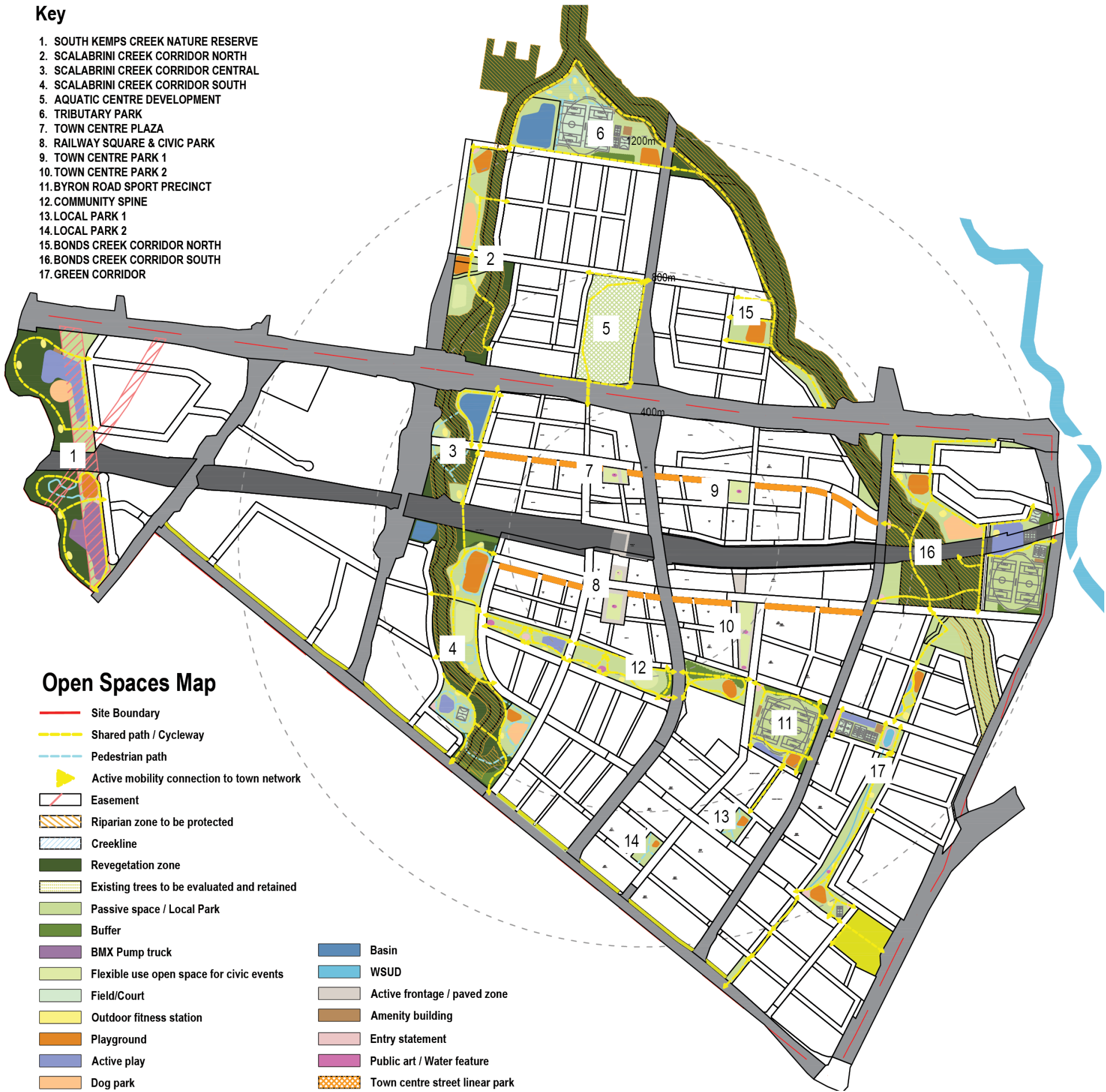
Figure 15 Leppington Town Centre Open Space Network
