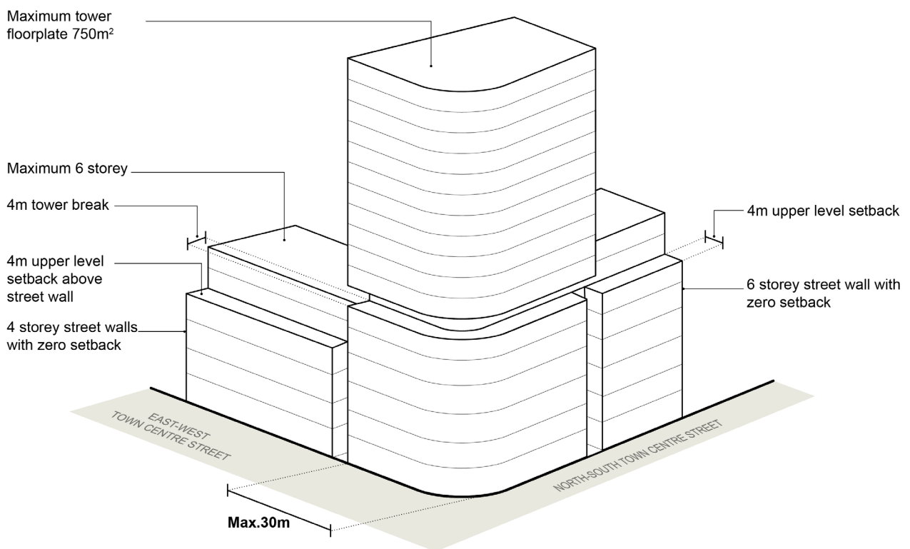
Figure 34 Zero setback with 4 or 6 storey street wall and 4m upper setback
