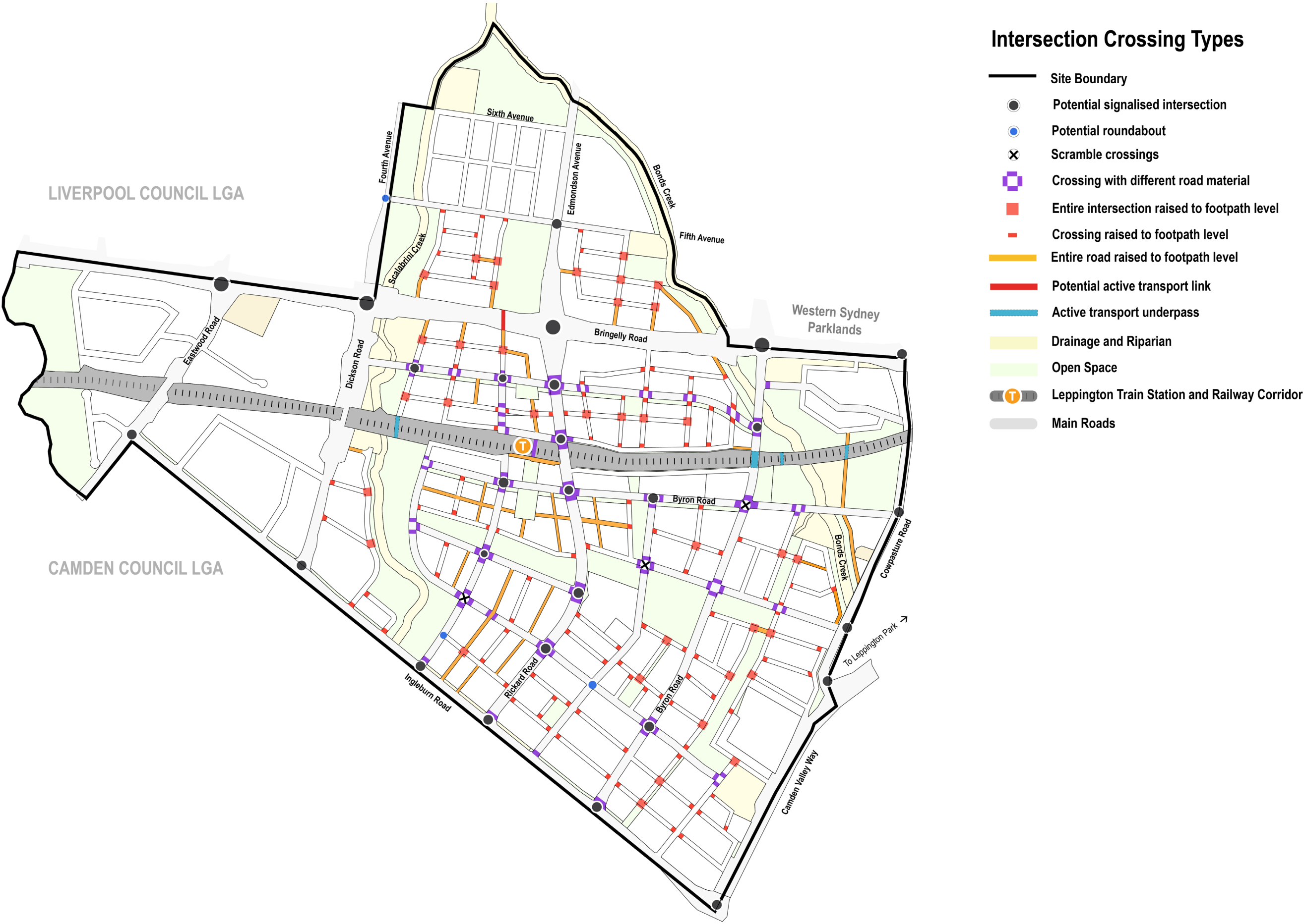
Figure 11 Intersection crossing types
