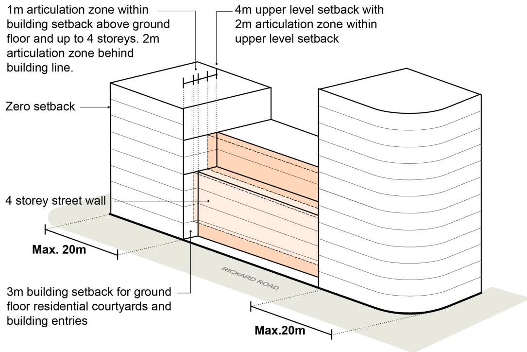
Figure 38 Rickard Road Residential (R4) setback and street interface
