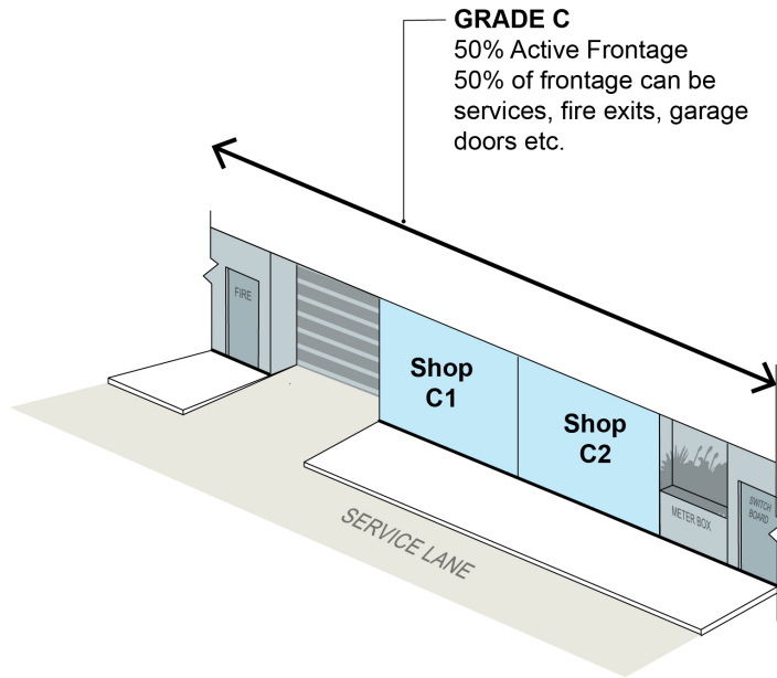
Figure 19 Grade C Commercial Frontage Axonometric
