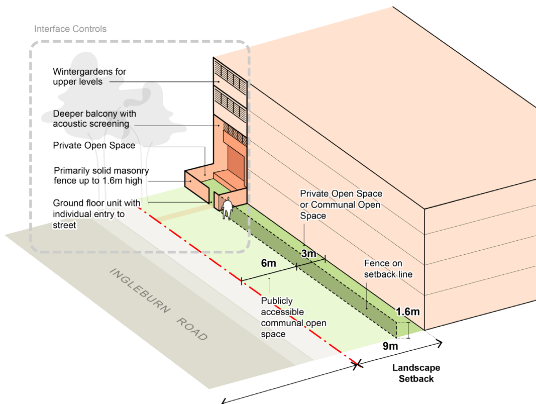
Figure 39 Ingleburn Road setback and street interface
