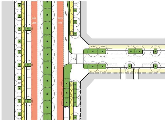
Figure 7 Raised pedestrian and cycle crossing
