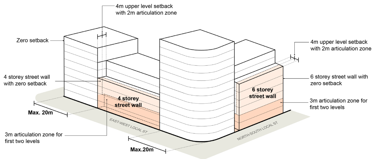
Figure 37 Residential (R4) Setback
