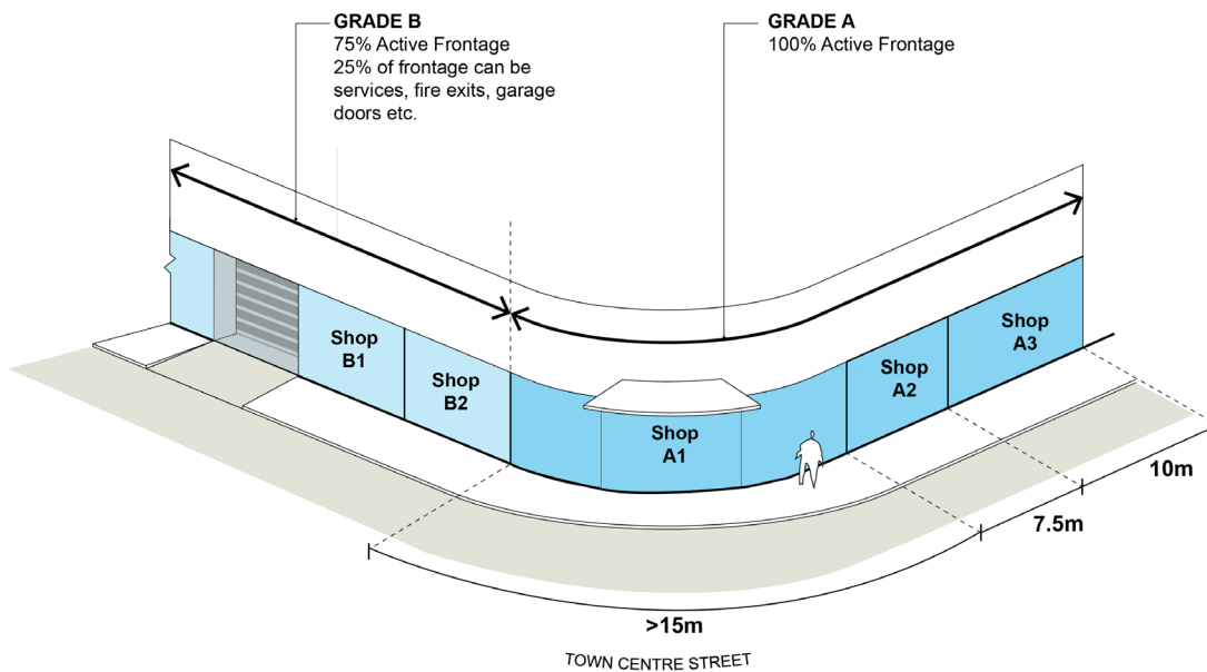
Figure 17 Grade A and B Commercial Frontage Axonometric
