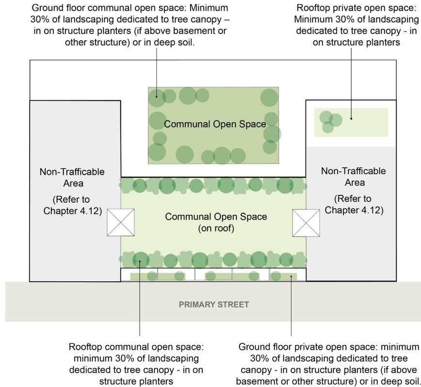
Figure 49 Tree canopy cover – Shop-top housing / apartments
