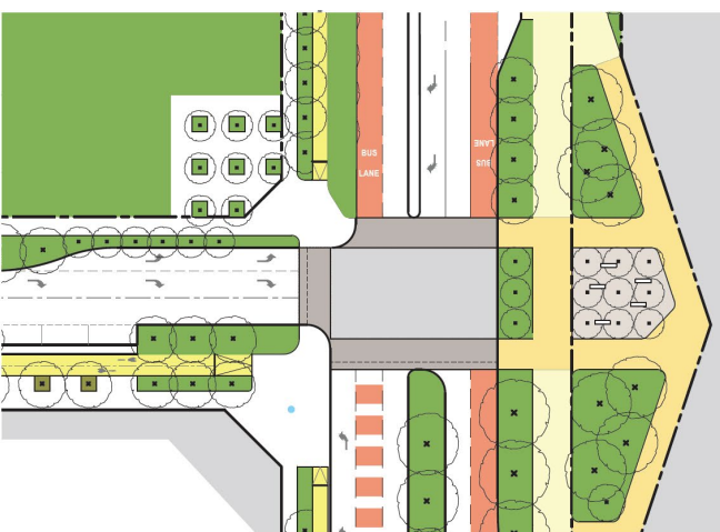
Figure 10 Special paving treatments to signalise intersections (different road material)
