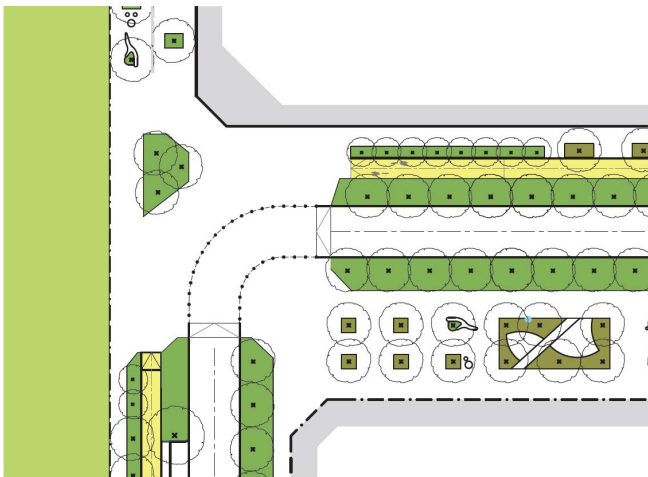
Figure 9 Raised pedestrian crossing on bend to connect plazas
